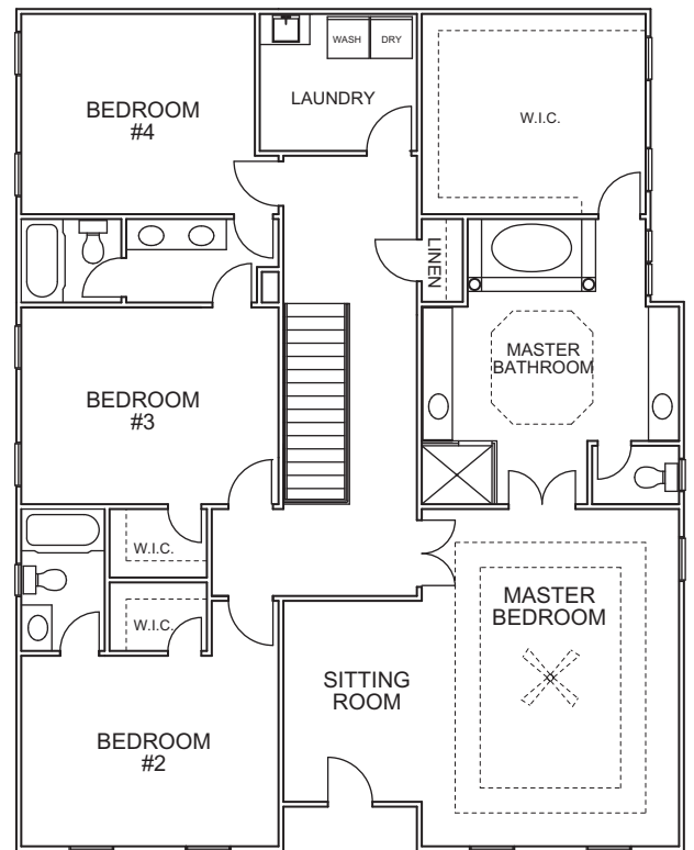
Second Floor
